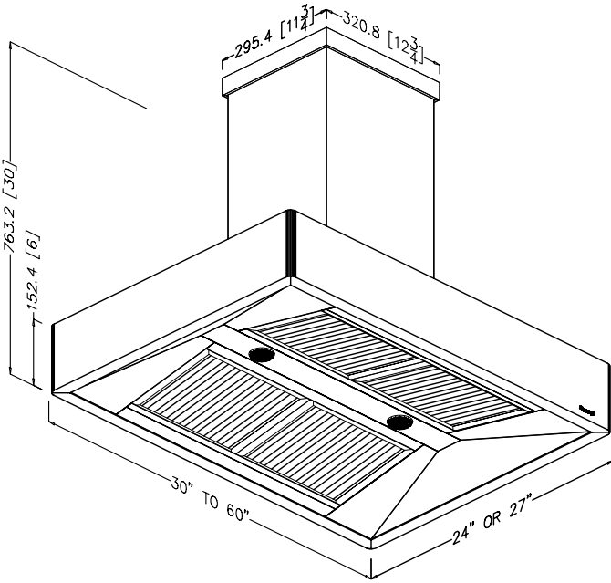
ISO VIEW
