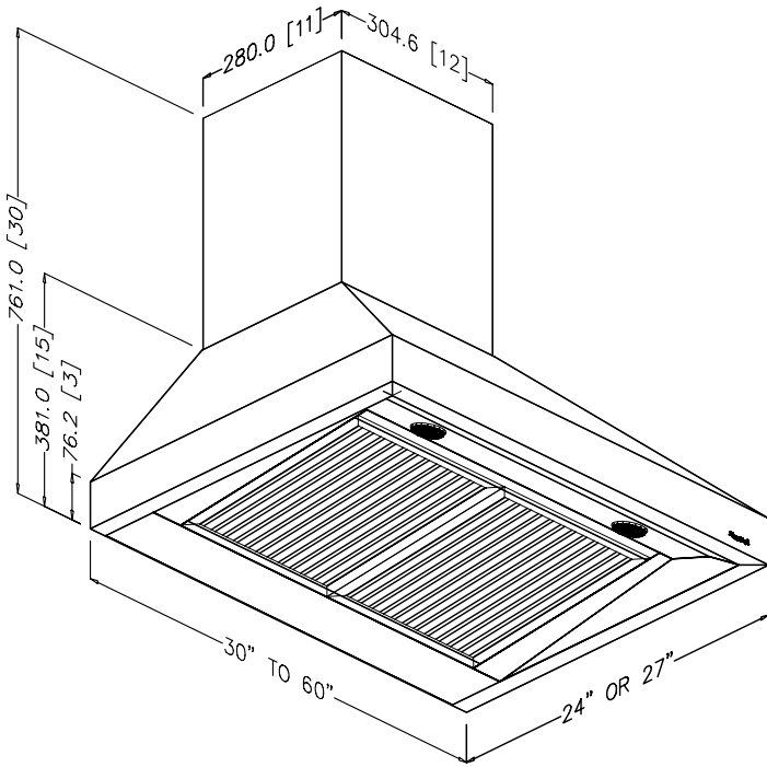
ISO VIEW
