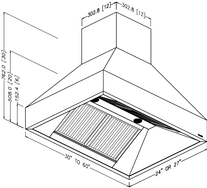
ISO VIEW
