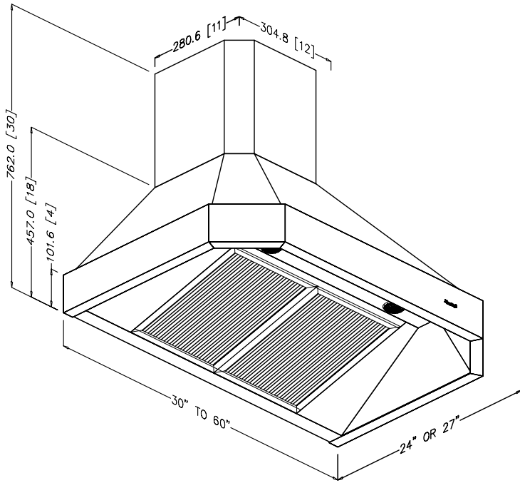
ISO VIEW
